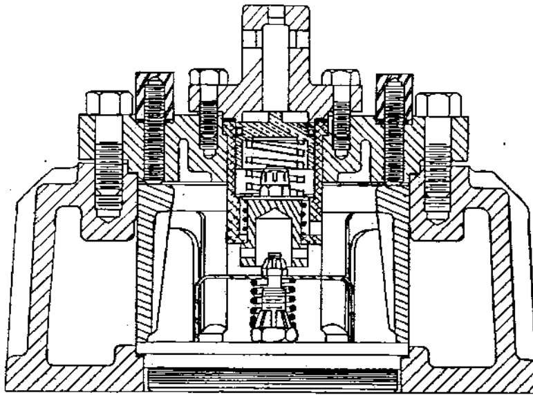
ASSEMBLY - SUCTION
